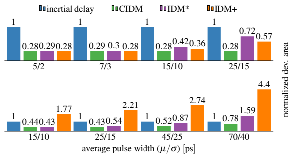
Figure 7: Accuracy, expressed as the normalized total deviation area of the digital predictions, relative to SPICE for the standard inverter chain (top) and high/low threshold inverter chain (bottom). Lower bars indicate better results.
