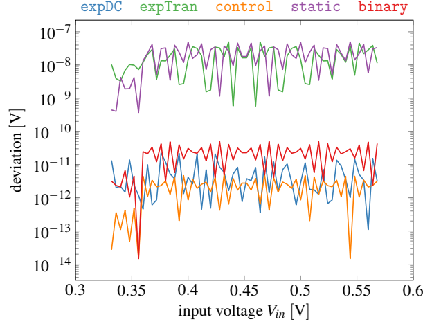
Figure 5.17: Absolute deviation between V_M predicted by various approaches compared to analytic calculations for opamp .
