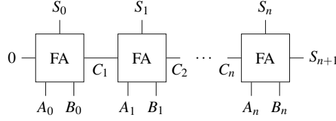
Figure 4.31: Adder gate level implementation.
