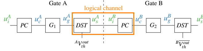
Figure 4.48: Channel model for proofs of the CIDM. Signals in blue have data type WST, those in green TCT.
