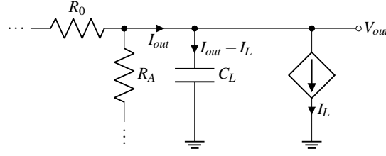
Figure 5.19: Circuit setup to characterize the linearized system dynamics and to over-compensate the current flow into the load capacitance.
