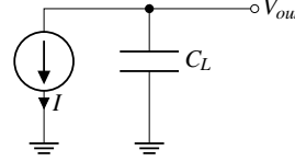
Figure 4.25: Inverter in Region 3).
