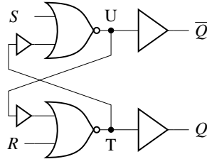
Figure 4.30: SR Latch gate level implementation.
