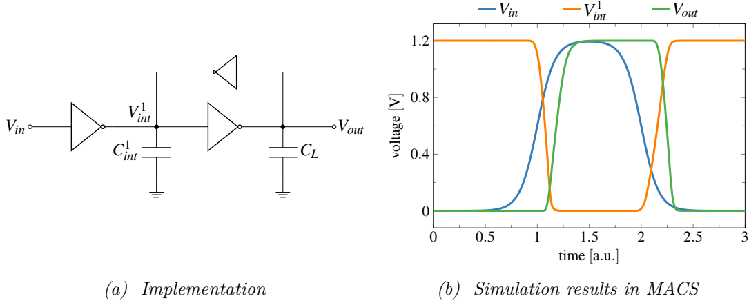
Figure 3.12: Memory element (D-latch) modeled using the Uniform Model. The internal capacitance C_{int}^1 is required to evaluate the voltage value at this point, whereat we used C_L/C_{int}^1 = 2 .
