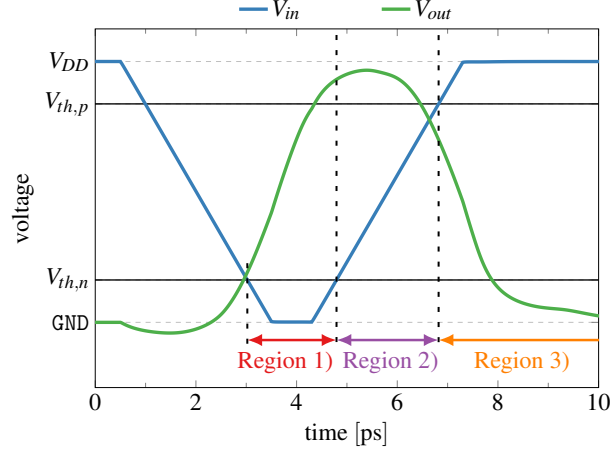
Figure 4.17: Overview of the Inverter operation regions in technology (T15) during switching. V_{th,n} respectively V_{th,p} represent the threshold voltages for n- and pMOS.
