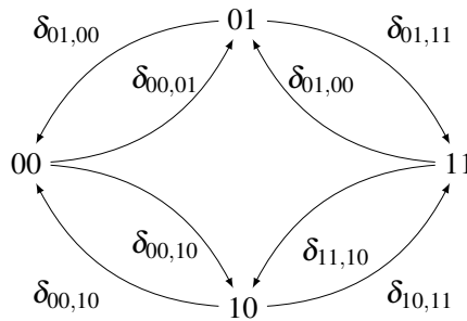
Figure 6.6: Interconnections of delay functions of Multi Input gates.
