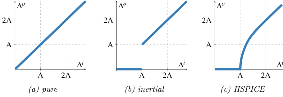
Figure 4.1: Output ( \Delta^o ) over input ( \Delta^i ) pulse-width of a single in- and output gate for the pure and inertial delay model compared to HSPICE simulations of a real circuit. The continuous degradation can not be modeled using those simple approaches.
