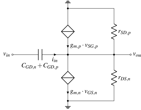
Figure 4.14: Simplified small signal representation of an Inverter using a current source (controlled by V_{Gy} ) and a resistor to model each transistor. v_{in} denotes the small displacement around the operating point V_{in} .
