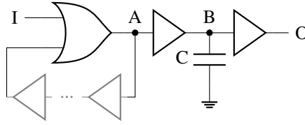
Figure 4.29: OR Loop gate level implementation.
