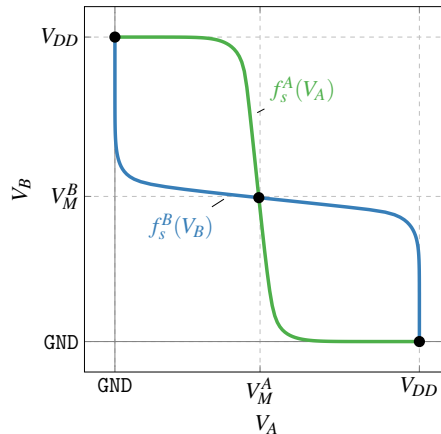
Figure 5.3: Static transfer characteristic f_s of the forward and backward Inverter in Latch #2 of Figure 5.2. The black dots mark the two stable configurations at the outskirts and the metastable one in the middle.
