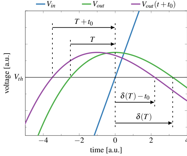
Figure 4.22: Shifting the cubic approximation of V_{out} by t_0 causes an increase in T and a decrease in \delta . The slope of the input signal V_{in} is approximated.
