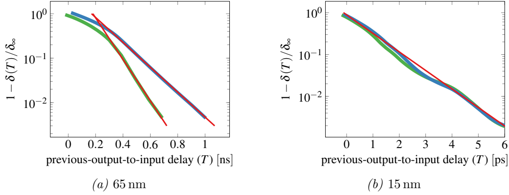
Figure 4.27: DDM delay function of the first Inverter for different technologies in logarithmic space with linear fitting.
