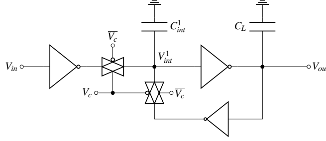
Figure 5.4: Uniform Model implementation of a Latch using Transmission gates.
