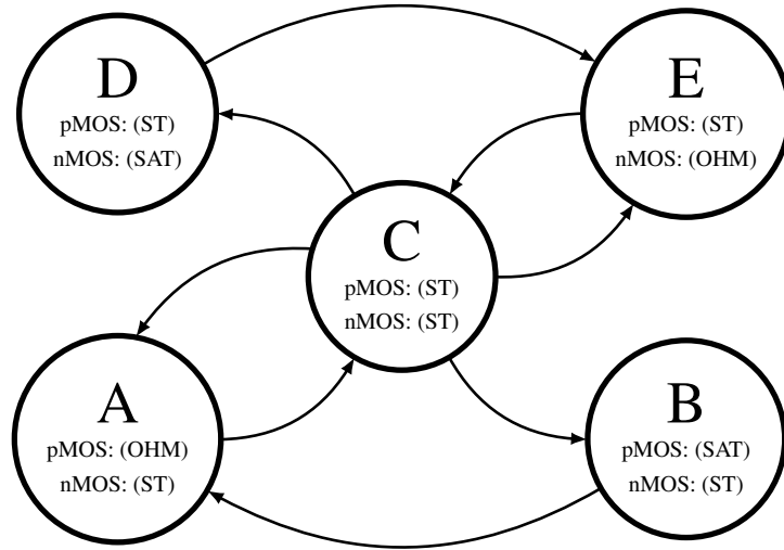
Figure 3.11: Graphical representation of the hybrid Inverter model for the case that V_{th,n} > V_{DD} - V_{th,p} . In each state, represented by a node showing the operation regions of the transistors, one of them has to be in (ST). Thus the number of possible states is reduced.
