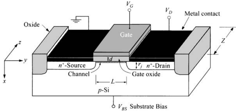
Figure 2.7: Internal structure of a FET. On top of the inner layer of an NPN structure, separated by a thin insulator, resides the gate, which controls the conductivity of the underlying channel. From [73, p. 298]
