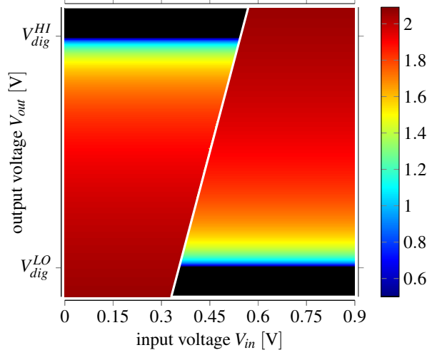
Figure 5.22: Resolution time \log_{10}(t_{res}/t_0) , t_0 = 1 ps for opamp in the V_{in} - V_{out} plane.
