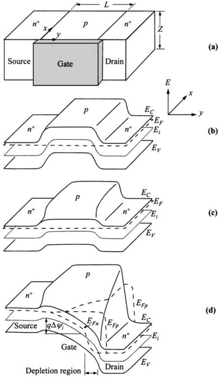
Figure 2.8: Band diagrams of the FET for (b) no gate voltage, (c) considerable gate voltage and (d) additional drain-source voltage. Taken from [73, p. 299]
