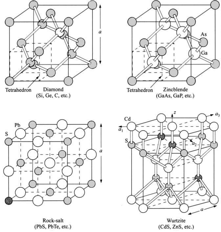
Figure 2.2: Primitive cells of various lattice structures. a denotes the lattice constant. For the Wurtzite structure the lattice constants differ between spatial directions. Taken from [73, p. 9].
