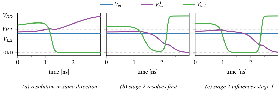
Figure 5.37: Analog simulation results for resolving from metastability in the cascade. We observed an upstream coupling in (c) where the resolution of stage 2 causes stage 1 to switch from approaching V_{DD} to GND.
