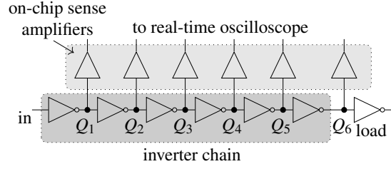
Figure 4.42: Schematics of the ASIC used for validation measurements. It combines an Inverter chain with analog high-speed sense amplifiers.
