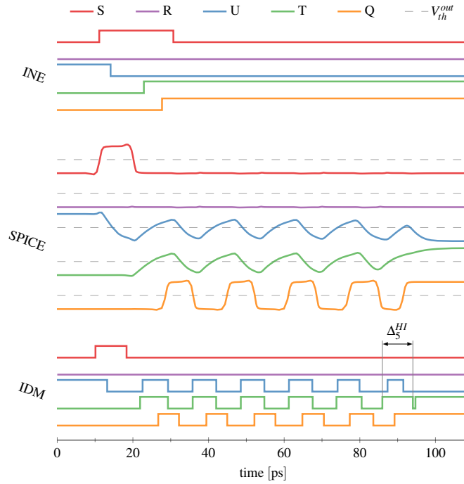
Figure 4.36: Analog and digital simulation showing metastability in the SR Latch.
