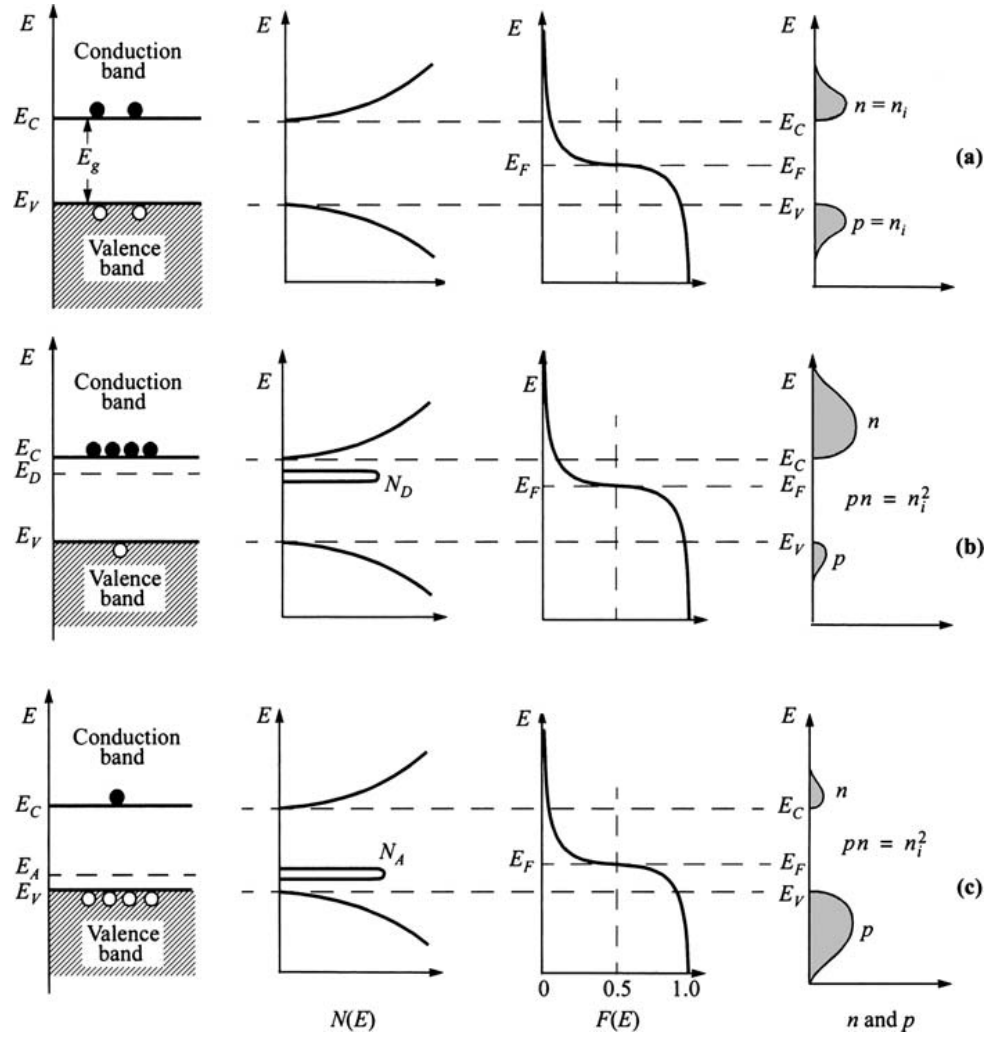
Figure 2.4: Band diagram for an (a) intrinsic, (b) n-type doped and (c) p-type doped semiconductor. N(E) shows the density of states and F(E) the distribution function. Please note that the product of electrons and holes is constant in all cases, i.e., n \cdot p = n_i^2 . Taken from [73, p. 24]
