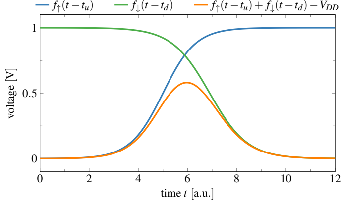
Figure 3.31: Creating pulses by properly adding shifted versions of the FRSWs. In this figure sigmoids were used. For t_d - t_u > 0 an up pulse is created, otherwise a down one. For asymmetric FRSWs, values below GND/above V_{DD} due to incorrect time shifts might appear, which have to be handled with care.
