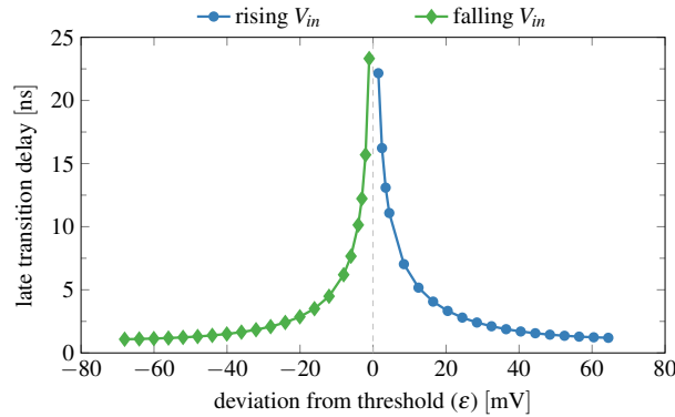
Figure 5.28: Late transition delay for rising and falling V_{in} stopping in distance \varepsilon above V_H / below V_L . The closer to zero the longer the delay with a pole at \varepsilon = 0 .
