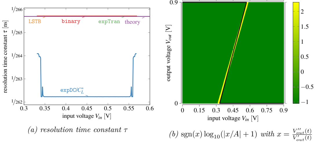
Figure 5.21: Results for opamp showing (a) the resolution time constant \tau along \gamma_2 and (b) the output behavior in the whole V_{in} - V_{out} plane.
