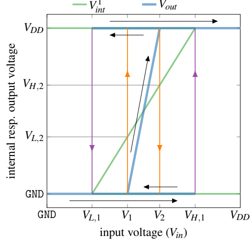
Figure 5.34: Theoretical analysis of the (meta-)stable states for the first S/T (green) and the cascade of two (blue). While the threshold points of the cascade are equal to the values of the first S/T (purple lines) with reversed direction, the metastable line \gamma_2 got much steeper since metastability is only possible when V_{int}^1 is driven between V_{H,2} and V_{L,2} . The orange lines, which indicate a resolution of stage 2, must not be crossed to keep the cascade in metastability.
