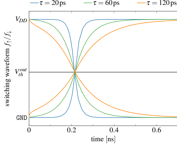
Figure 4.15: Different switching waveforms matching the same delay functions. The pieces after crossing V_{th} are initially fixed for varying time constant. Less steep ends lead to steeper beginnings.
