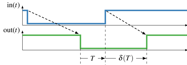
Figure 4.2: Delay estimation in a single history model. The delay \delta is determined based on the parameter T , which is defined as the time difference between the current input transition and the previous output one.
