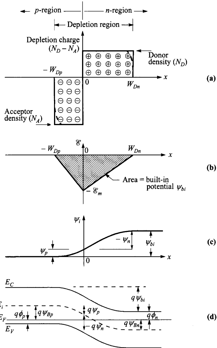
Figure 2.5: (a) Charge distribution, (b) electric field, (c) potential distribution and (d) band diagram of a p-n junction. Please note the asymmetries due to differing doping of p- and n-material. In this case the former is higher doped. Taken from [73, p. 80]
