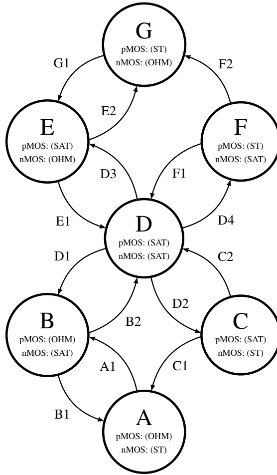
Figure 3.10: Graphical representation of the hybrid Inverter model. Each node represents a single state which is identified by the operation regions of the n - and p MOS.
