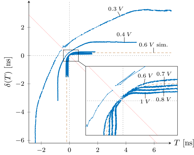
Figure 4.43: Measured \delta_{\downarrow} for UMC-90 Inverter chain for V_{DD} \in \{0.3, 0.4, 0.6, 0.7, 0.8, 1\} V and simulated (dashed brown) \delta_{\downarrow} for V_{DD} = 0.6 V, taken from [38, Fig. 7].
