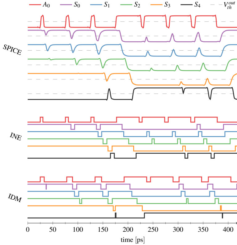
Figure 4.38: Analog and digital simulation of the Adder with a glitch on its input.
