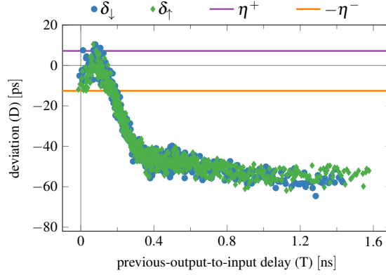
Figure 4.45: Fitting an Exp-channel involution to measured data. For small values of T the \eta -bounds are sufficient to cover the deviations.
