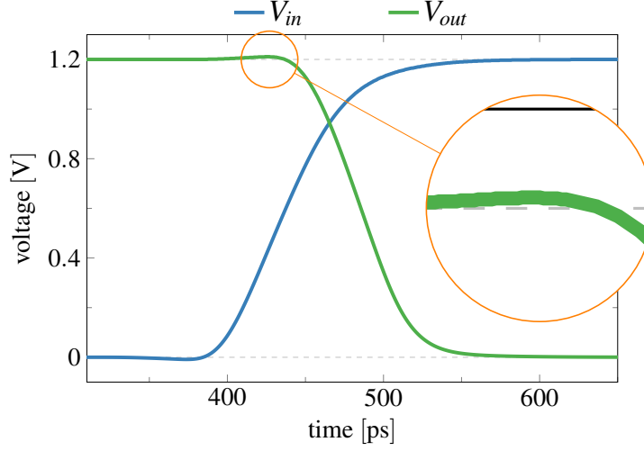
Figure 3.6: Dynamic HSPICE switching behavior of a CMOS Inverter in technology (T65). For this simulation an Inverter chain with capacitive load was used to properly shape the pulses. The figure shows input and output of the fifth Inverter. Please note the over/undershoot before the actual transition.
