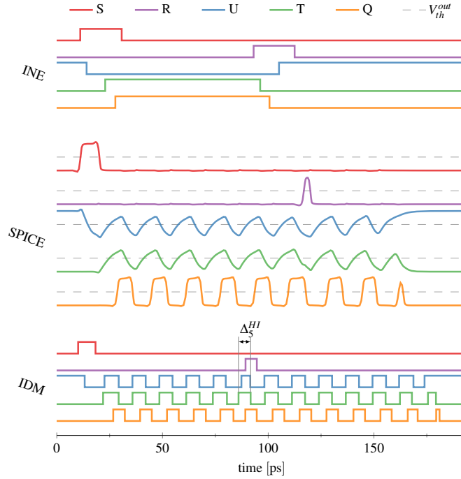
Figure 4.37: Analog and digital simulation of keeping the SR Latch in metastability.
