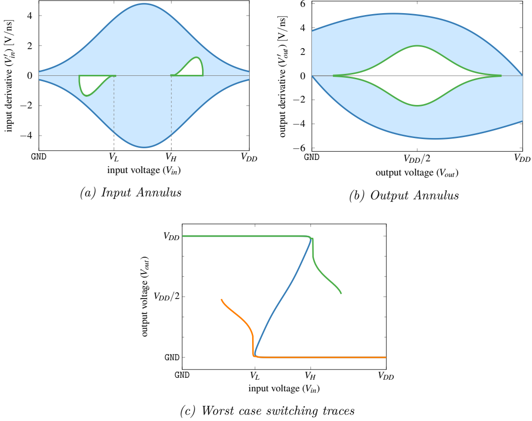
Figure 5.39: Results of our approach that determines the possible input behavior to prevent metastability in an S/T while fulfilling specific output requirements. Note that the tool is still under construction and not published yet.
