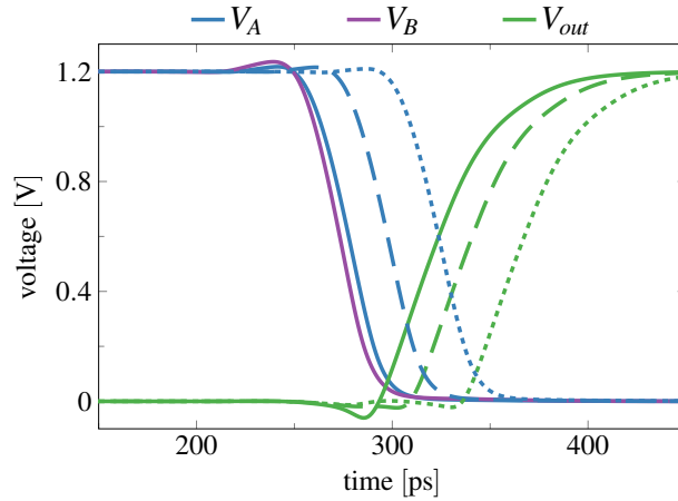
Figure 3.15: HSPICE simulations for a rising output transition of a NOR gate in technology (T65). Two values of \Delta are used. The shape of the output waveform stays constant, it solely shifts in time.
