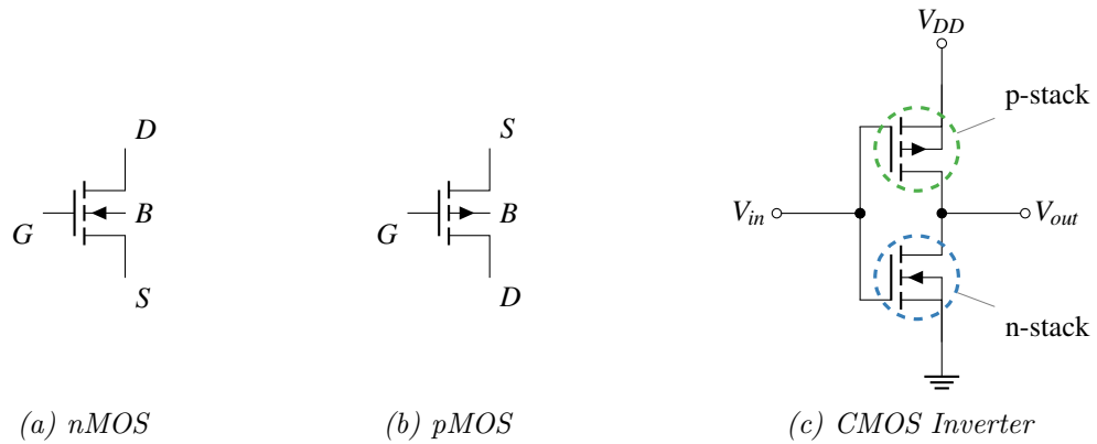
Figure 2.13: Transistor symbols used in circuit schematics for nMOS (a) and pMOS (b). Combining both results in an Inverter (c).
