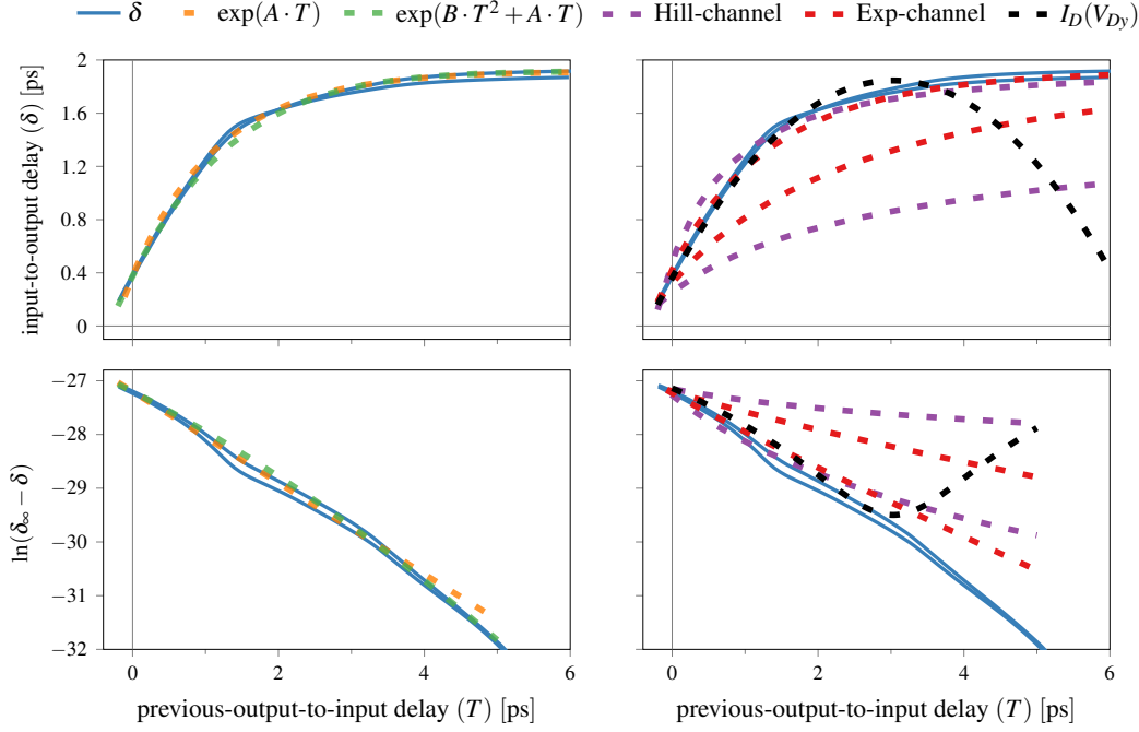
Figure 6.2: Multiple approaches to fit the IDM delay function of a place \mathcal{E} routed Inverter using technology (T15) on a linear (upper) and logarithmic (lower) scale. The exponentials on the left side are only fit to one delay function since \delta_\uparrow and \delta_\downarrow differ solely marginally.
