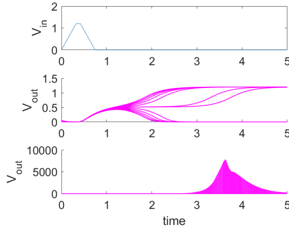
Figure 5.8: Metastability analysis of an OR Loop in C2E2 using technology (T65). For a single input pulse (top) significantly different simulation traces (middle) have been achieved by changing the initial value of V_{out} minorly. The reachtube (bottom), corresponding to the trace sticking longest in metastability, reaches unreasonable high values, which indicates a very high sensitivity.
