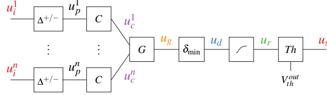
Figure 4.47: Channel model for CIDM.
