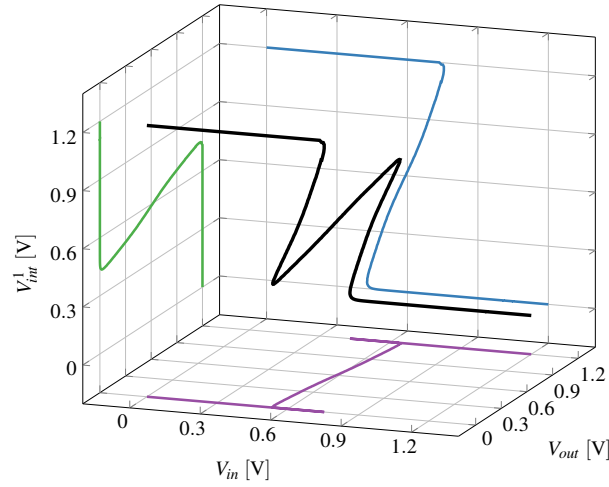
Figure 5.35: Phase plane representation of the cascade in three dimensions. The single faces show the characteristic for each single stage and the combined one.
