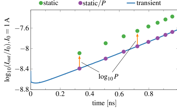
Figure 5.14: Comparison of the output current for transient and static simulations.
