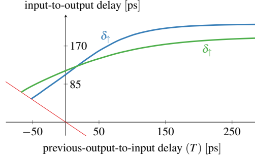
Figure 4.13: Characterizing a gate with V_{th}^{in} = V_{th}^{out} = V_{DD}/2 . Clearly visible are the differing pure delay components \delta_{min}^{\uparrow} \neq \delta_{min}^{\downarrow} .
