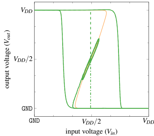
Figure 5.30: Phase space representation for the output waveform presented in Figure 5.29. During the sine wave behavior the trace sticks closely to \gamma_2 (orange line).
