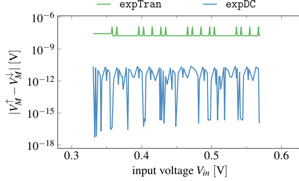
Figure 5.16: Absolute deviation between V_M predictions for resolution towards V_{DD} ( V_M^\uparrow ) and GND ( V_M^\downarrow ).
