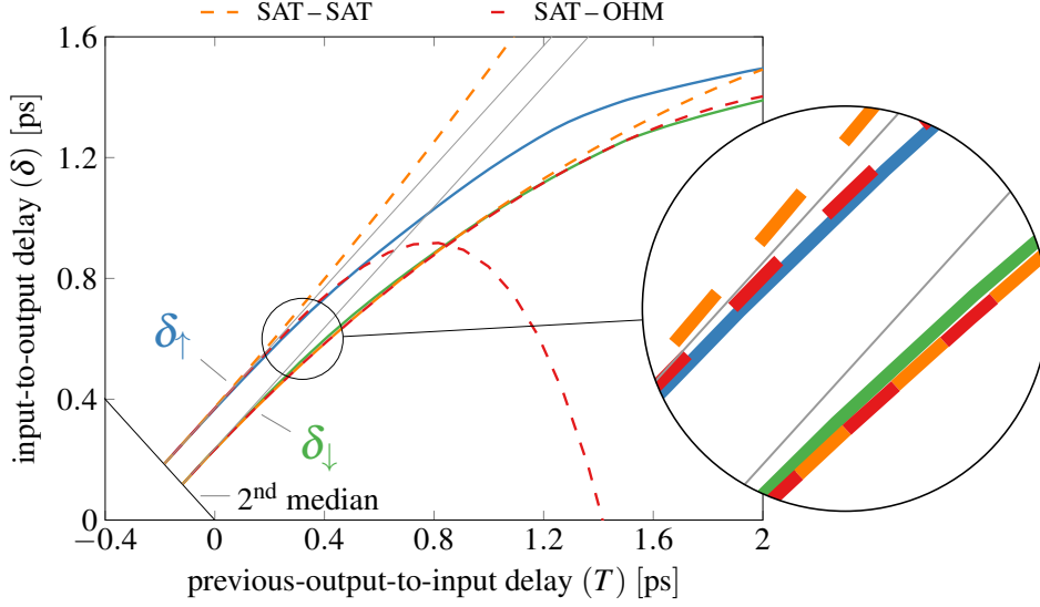
Figure 4.21: DDM delay function of the first Inverter in the 15 nm Inverter chain (solid lines) vs. predictions based on our simplifications (dashed lines).
