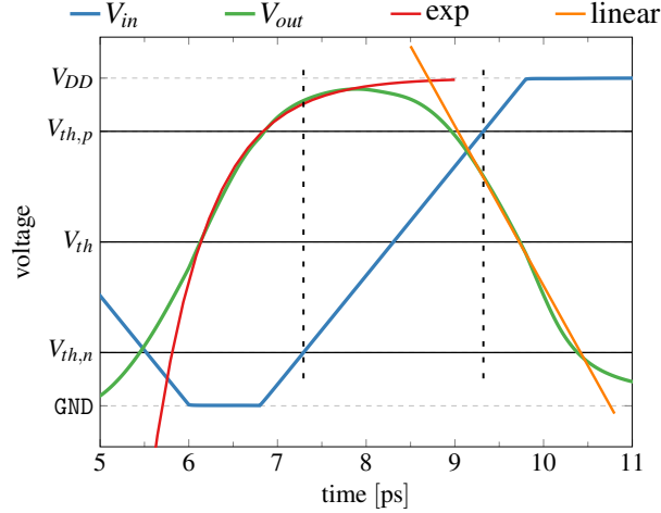
Figure 4.26: Simplification of V_{out} for Region 1) & 3) for 15 nm technology. The exponential increase is followed by a linear drop.
