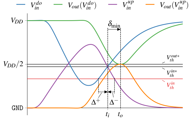
Figure 4.12: The unique relationship among V_{th}^{in*} , \delta_{\min} and V_{th}^{out*} for a Buffer based on simulations in technology (T15).
