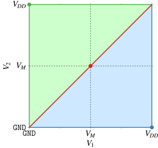
Figure 3.30: Convergence Plane for starting values V_1 and V_2 of the Inverter loop. For all points in the blue area the stable point (V_1, V_2) = (V_{DD}, GND) is approached, while for the ones in the green area (V_1, V_2) = (GND, V_{DD}) is achieved. A special case are the points on the red line V_1 = V_2 , which end up in (V_1, V_2) = (V_M, V_M) .
