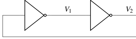
Figure 3.28: Layout of an Inverter loop used to simulate pulses using InvUni .
