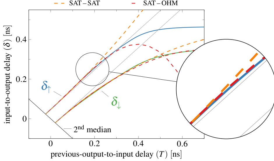
Figure 4.20: DDM delay function of the first Inverter in the 65 nm Inverter chain (solid lines) vs. predictions based on our simplifications (dashed lines). Clearly visible is the super-linear growth of \delta_{\uparrow} for T < 0.2 ns.
