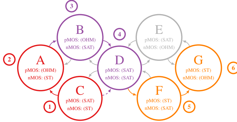
Figure 4.18: Transition graph of the transistor operation regions in an Inverter. The first line in a node shows the pMOS, the second one the nMOS. The colors correspond to Region 1) [red], 2) [purple] and 3) [orange].
