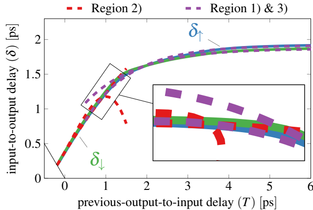
Figure 4.28: Fitting of the involution delay function for the seventh Inverter in the 15 nm chain.
