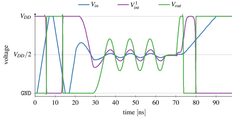
Figure 5.36: “Arbitrary” waveform derived by operating both S/Ts in metastability. After the initial normal operation a sine wave is enforced at the output. Note the amplification in this region, causing a rather small swing on V_{in} having large effects on V_{out} . In the end separate resolution of the single stages can be observed for a linear input.
