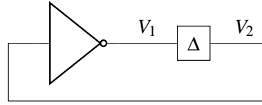
Figure 3.26: Simulation setup for determining f_{\uparrow} and f_{\downarrow} of the Inverter. The pure delay component \Delta is required to achieve a reasonable time distance between succeeding transitions, such that interference (pulse creation) can be avoided.
