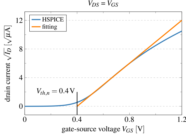
Figure 2.9: Square root of the drain current \sqrt{I_D} through a 65 nm n MOS over V_{GS} ( V_{DS} = V_{GS} ). The threshold voltage V_{th,n} was determined by a linear extension in the point with the highest derivative.
