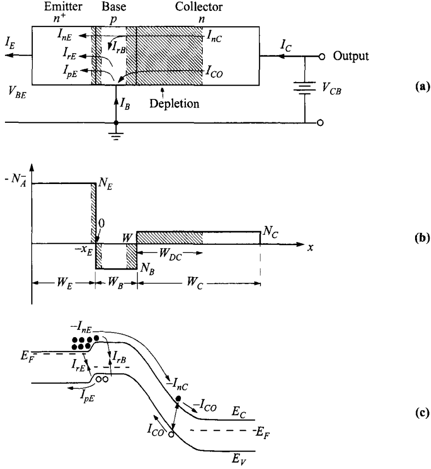
Figure 2.6: (a) Internal Structure, (b) doping profile and (c) band diagram of a bipolar transistor. The base-collector diode used in reverse direction collects (most of) the charge carriers injected by the emitter-base diode, which is driven in forward direction. Taken from [73, p. 246]
