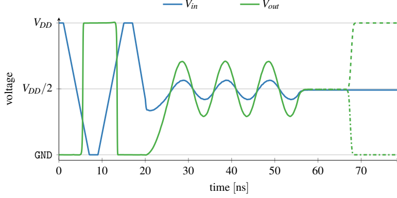
Figure 5.29: Creating an arbitrary waveform at the output of the S/T. After an initial phase a sine with a frequency of 100 MHz is created. Note that, albeit looking that way, V_{out} does not follow V_{in} in this phase. Instead V_{in} is used to slow the output down. In the end the S/T is allowed to resolve starting from minorly differing values.
