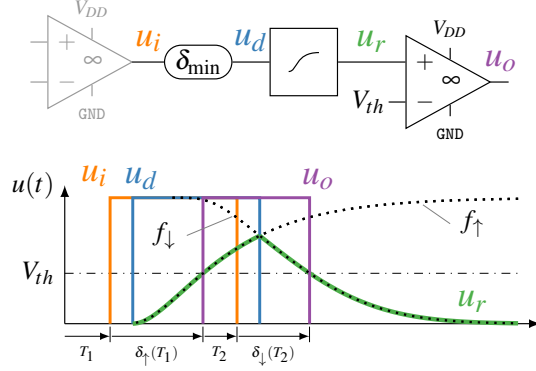
Figure 4.8: Simple analog channel model (upper part) with a sample execution (bottom part). The switching from f_{\uparrow} to f_{\downarrow} is done instantly when a transition on u_d arrives, leading to continuity in u_r but a jump in its derivatives. Heavily inspired by [34].
