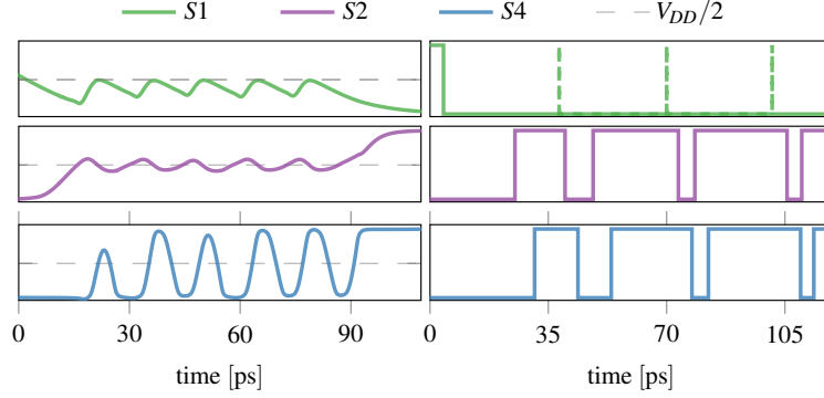
Figure 4.51: Analog and digital prediction of recovering sub-threshold waveform.
