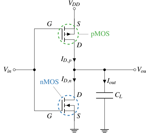
Figure 3.4: CMOS Inverter implementation on the transistor level, consisting of a pMOS (top transistor) and nMOS (bottom transistor). Their respective drain currents I_{D,n} and I_{D,p} are used to determine I_{out} , which (dis)charges the load capacitance C_L and thus determines V_{out} .
