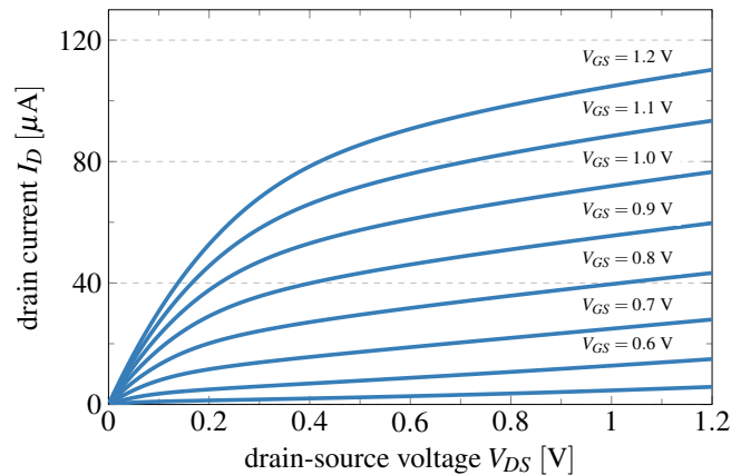
Figure 2.10: HSPICE simulations of the drain current I_D through a 65 nm nMOS over V_{DS} for different values of V_{GS} . The deviating behavior in (OHM) and (SAT) is clearly visible, however, a unique separation is not easily possible.
