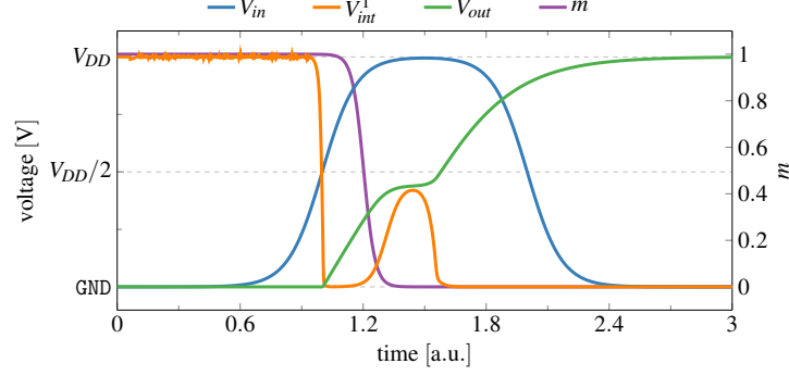
Figure 5.6: Simulation of the Latch in metastability using MACS. By varying the transition time of m(t) , which models the Transmission gates, longer metastable states (flat part of V_{out} ) can be achieved.
