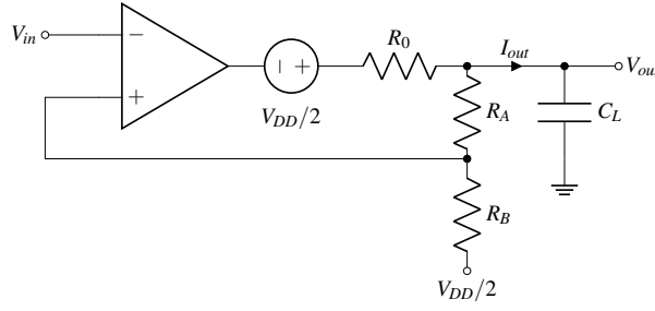
Figure 5.12: Circuit level implementation of opamp.
