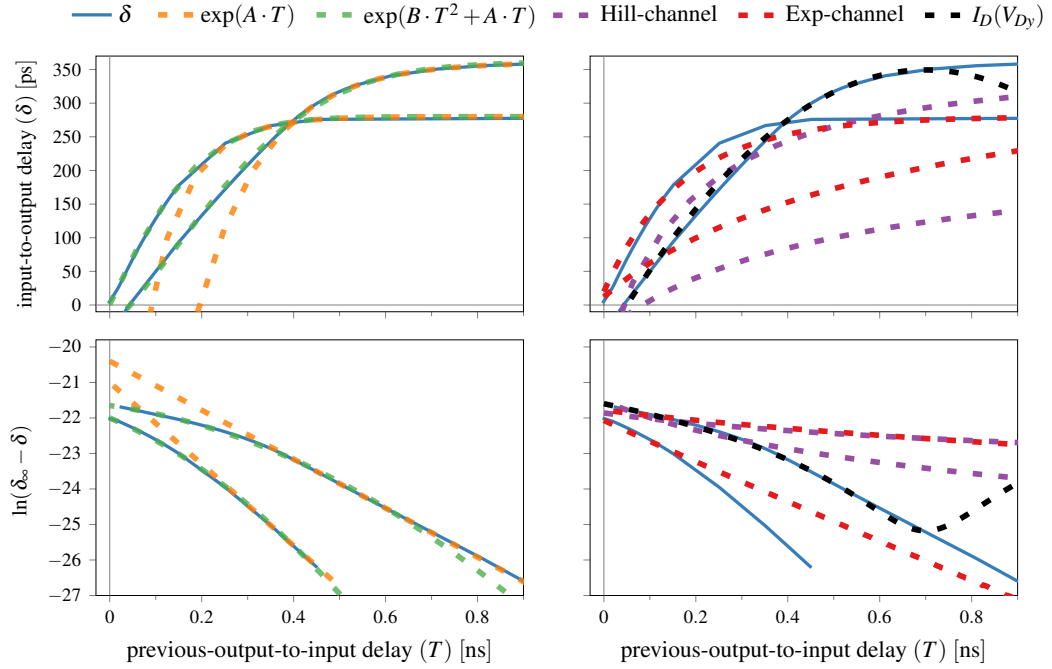
Figure 6.1: Multiple approaches to fit the DDM delay function of an optimal Inverter on a linear (upper) and logarithmic (lower) scale.
