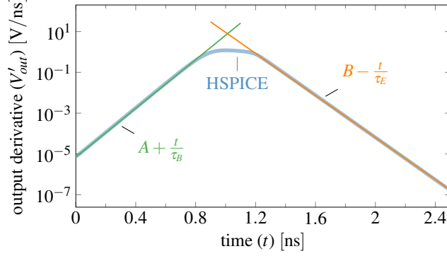
Figure 5.40: Resolving metastability of std for V_{in} = 0.64 V using technology (T65). The slopes can be very accurately modeled by an exponential approach.
