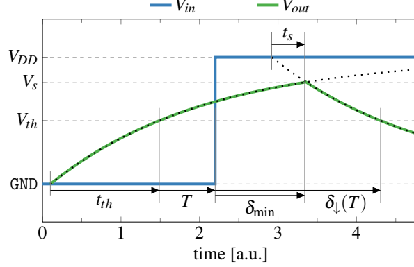
Figure 4.9: Graphical derivation of the IDM delay function. For finite values of T the downward switching waveform f_{\downarrow} does start at an intermediate voltage V_s = f_{\downarrow}(t_s) causing the time to reach V_{th} ( t_{th} ) to be reduced by t_s .
