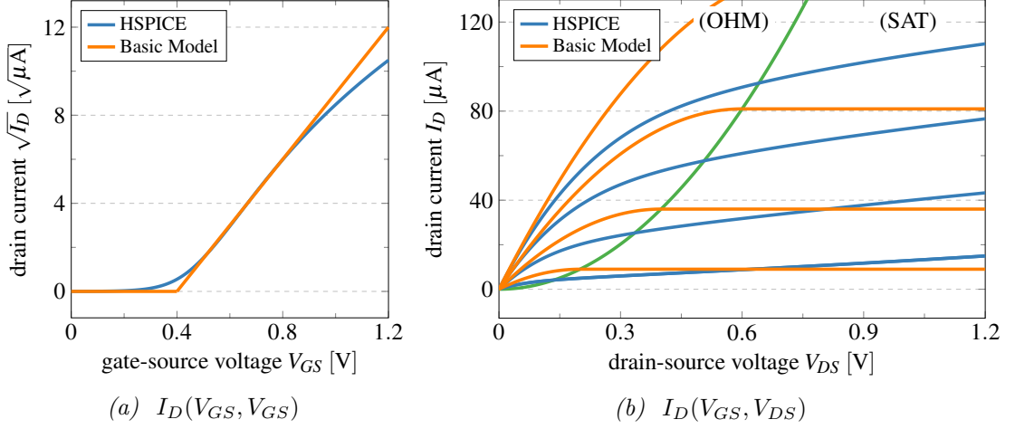
Figure 3.1: Basic Model approximations of the drain current I_D through an nMOS in technology (T65) (a) for V_{GS} = V_{DS} and (b) over V_{DS} for V_{GS} \in \{1.2, 1, 0.8, 0.6\} V. This simple model shows quite some deviations, especially for large gate-source voltages.
