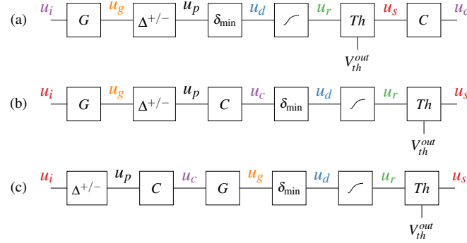
Figure 4.46: Candidate channel models for the CIDM.
