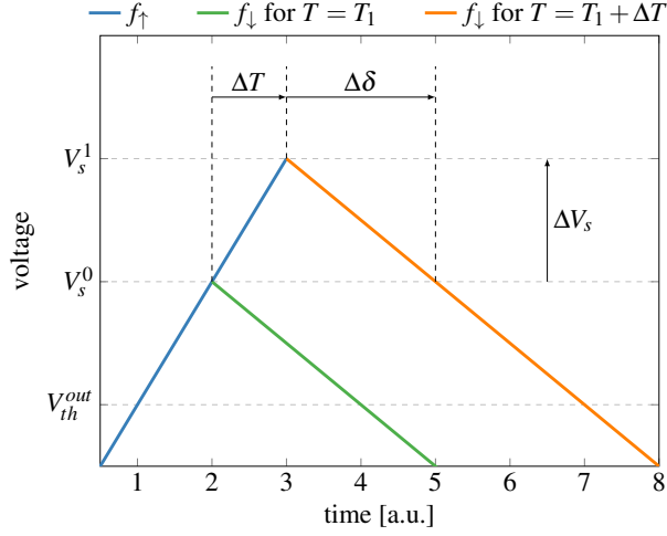
Figure 4.16: A linearized pulse barely exceeding V_{th} showing the difference in the delay based on the change of parameter T .
