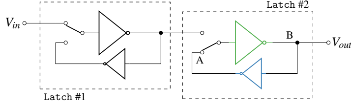
Figure 5.2: Internal structure of a Flip-Flop, consisting of two Latches in succession. Please note that the switches are controlled by the same signal such that one Latch stores a value while the other one propagates its input.
