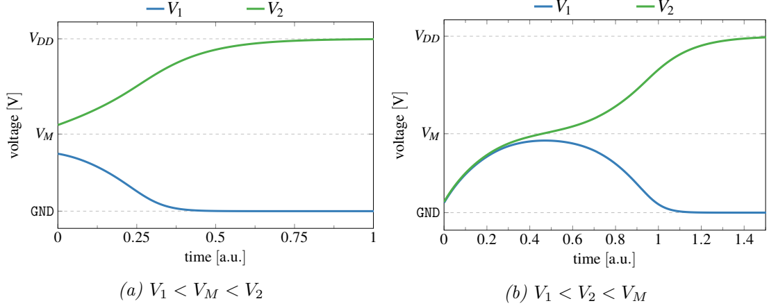
Figure 3.29: MACS simulations of the Inverter loop. Depending on the initial conditions either direct resolution (left) or pulse creation (right) can be observed.
