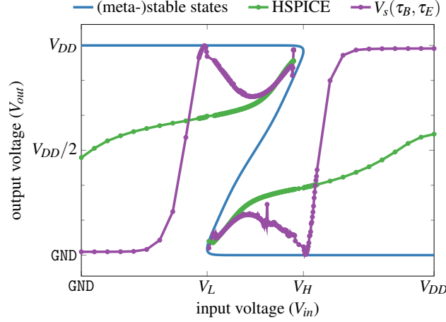
Figure 5.41: Resolution region crossing points ( V''_{out} = 0 ) once derived directly from HSPICE simulations and once predicted based on the fitted \tau_B and \tau_E . Obviously the latter is not yet a viable alternative.
