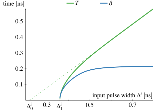
Figure 6.3: T and \delta of an Inverter using technology (T65) as functions of the input pulse-width \Delta^i . The combined delay function \delta(T) looks similar to the blue curve whereat the lower part is stretched along the x-axis.
