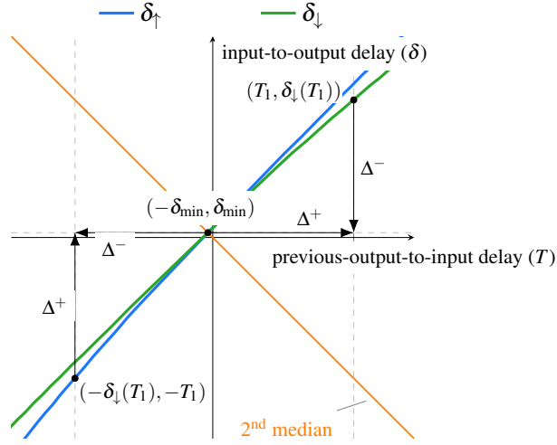
Figure 4.49: \Delta^+ and \Delta^- shown on the delay functions of gate A. Due to the mirroring along the 2 nd median the values once refer to \delta_\downarrow and once to \delta_\uparrow .
