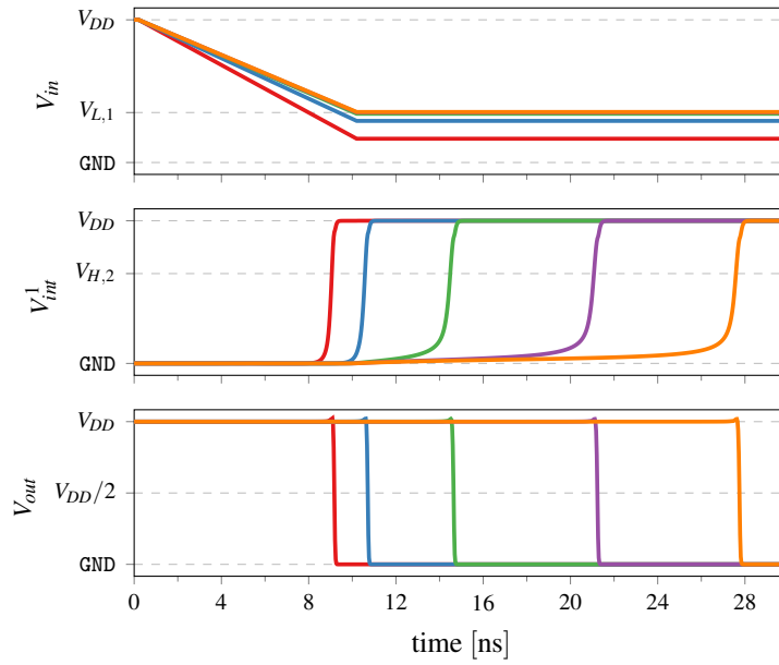
Figure 5.32: Analog simulations of V_{in} , V_{int}^1 and V_{out} for input slopes stalling at a constant value near V_{L,1} . Clearly stage 2 only increase the slope but leaves the transition time untouched.
