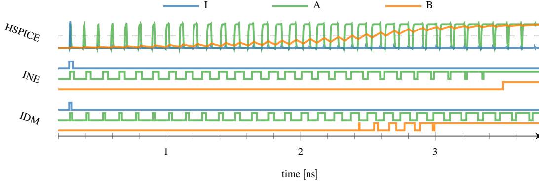
Figure 4.32: Analog and digital simulation results for the OR Loop with long feedback.
