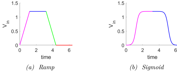
Figure 3.22: C2E2 input traces. The colors mark the different states of the automata. Note that for Sig only symmetric pulses are possible, i.e., where up and down transition have the same slope.
