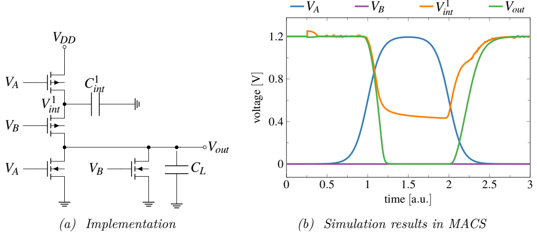
Figure 3.17: Implementation of a NOR gate in the Uniform Model and MACS simulation results for an SIS on input A. For the simulations a ratio of C_L/C_{int}^1 = 4 was used. V_{int}^1 shows some artifacts which are not visible in HSPICE simulations.
