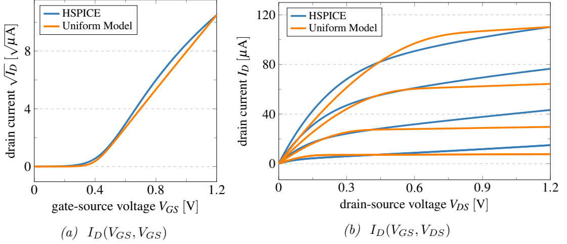
Figure 3.3: Uniform Model approximations of the drain current I_D through an nMOS in technology (T65) (a) for V_{GS} = V_{DS} and (b) over V_{DS} for V_{GS} \in \{1.2, 1, 0.8, 0.6\} V. The achieved results are very much comparable to the Elaborate Model.
