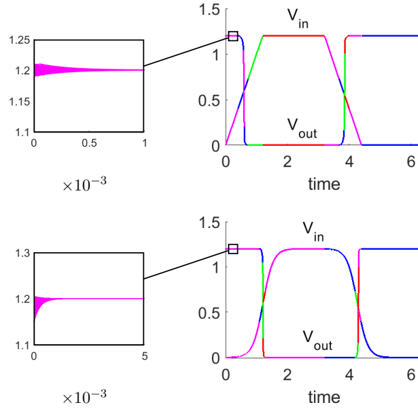
Figure 3.23: InvHy output voltage over-approximation set for V_{in} = \text{Ramp} (top) and V_{in} = \text{Sig} (bottom). Clearly visible are the states in V_{out} encoded by different colors.
