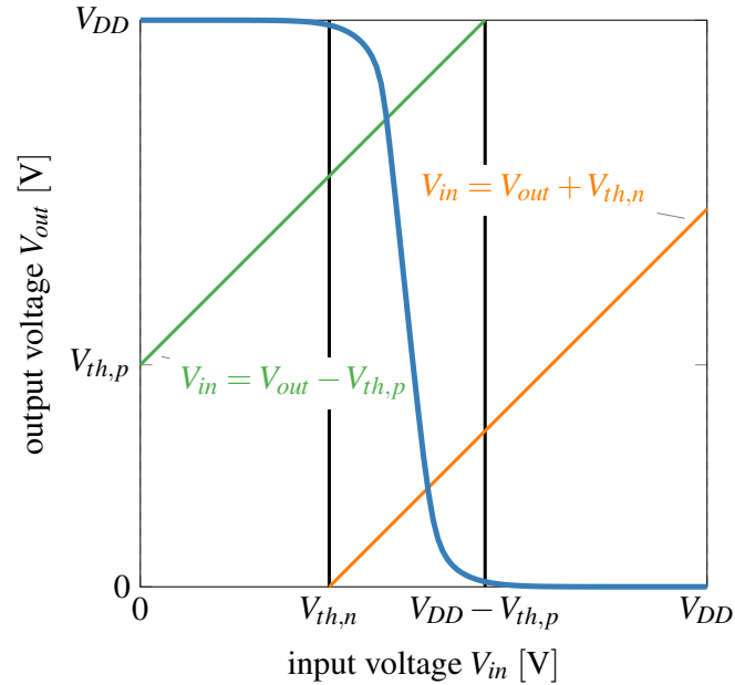
Figure 3.5: Transfer characteristic f_s(V_{in}) = V_{out} for a CMOS Inverter in technology (T65). Operation regions are determined using the Basic Model. In between the lines V_{out} - V_{th,p} , V_{out} + V_{th,n} and V_{th,n} < V_{in} < V_{DD} - V_{th,p} both transistors are operating in (SAT) such that the Inverter operates as a linear amplifier.
