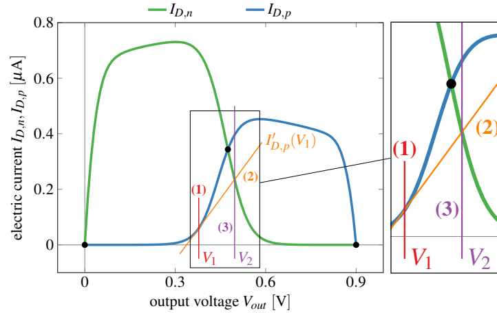
Figure 5.20: Application of the Newton-Raphson algorithm to find a statically stable V_{out} for fixed V_{in} (black dots).
