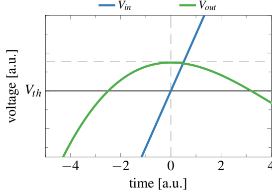
Figure 4.19: Cubic approximation of V_{out} . An arbitrary slope was chosen for V_{in} as k is hard to derive from the cubic function used for drawing the output curve.
