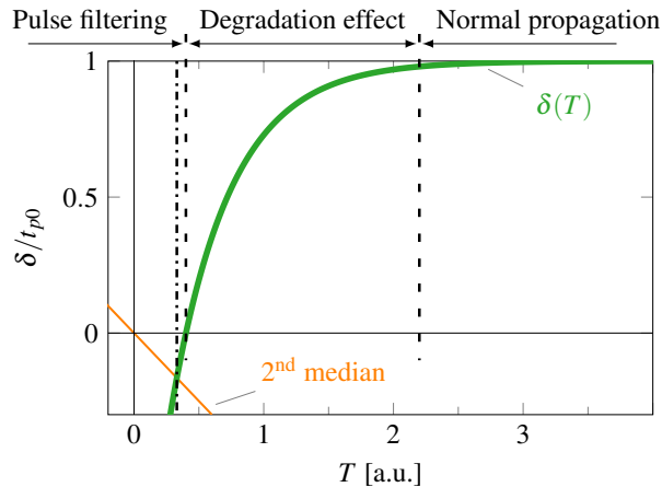
Figure 4.4: Exponential approximation for the DDM delay function \delta(T) . Different regions (dashed lines) are distinguished by the authors. We disagree with the onset of pulse filtering at \delta = 0 , which should be T = -\delta(T) marked by the dashed-dotted line. Heavily inspired by [82].
