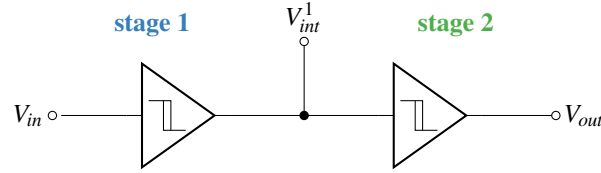
Figure 5.31: Two stage S/T cascade used in this thesis. We chose to use two inverting S/Ts, however, any combination of (non-)inverting ones are possible.
