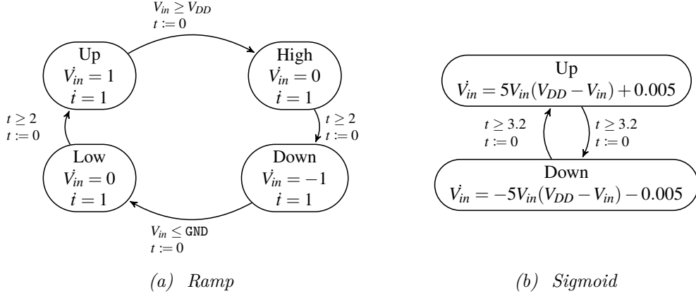
Figure 3.21: Input generation automata for C2E2.
