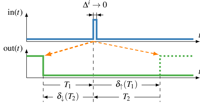
Figure 4.5: Proper cancellation of an input glitch ( \Delta^i \rightarrow 0 ) for a delay model. Since the glitch is supposed to have no impact on the output, the scheduled output transition (dotted line) has to be canceled, such that the previous output transition (solid line) is restored.
