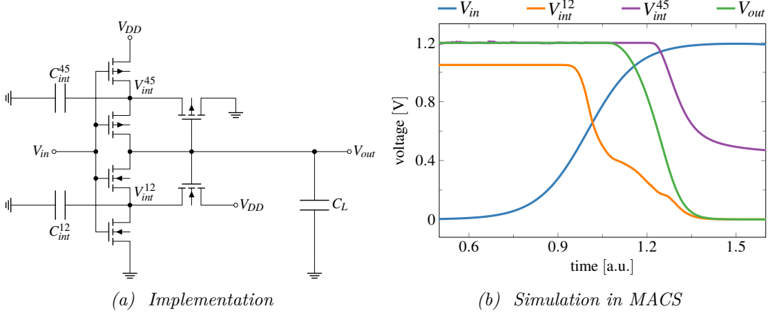
Figure 3.20: Uniform Model representation of the S/T with C_L/C_{int}^{12} = C_L/C_{int}^{45} = 4 . The results are in very good agreement to HSPICE simulations. V_{int}^{45} shows some simulation numerical artifacts.
