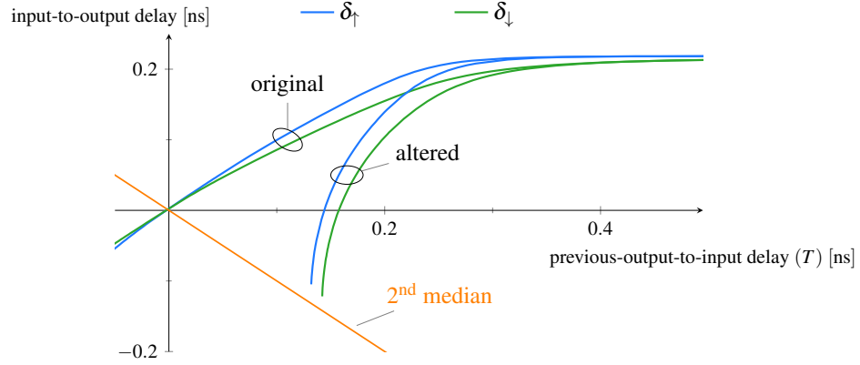
Figure 4.11: Correction of IDM delay functions to account for the non-constant delay of the first transition. In more detail, applying the altered delays results in more accurate output pulse-widths which are however still shifted in time. Please note the similarity of the altered \delta_{\uparrow} and \delta_{\downarrow} to DDM.
