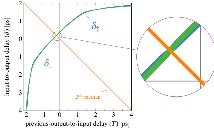
Figure 4.6: IDM delay function of an Inverter in technology (T15), numerically derived by extensive analog simulations in HSPICE.
