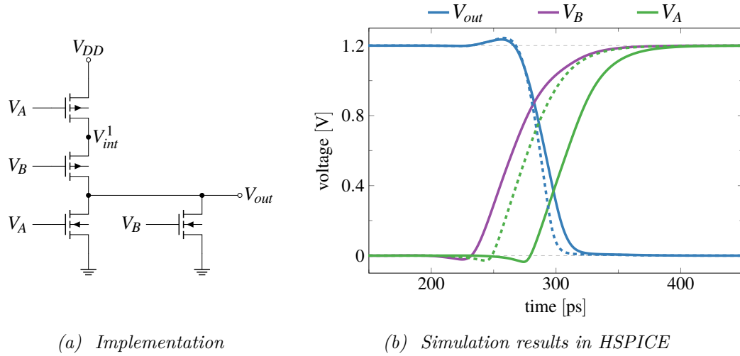
Figure 3.13: The CMOS NOR gate. Compared to the Inverter one n - and p MOS were added, whereat the former are in parallel and the latter in sequence. Simulations for Two values of \Delta show a much steeper output transition for the smaller one. Please note also the over-/undershoot, which we already analyzed for the Inverter.
