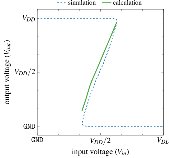
Figure 5.11: Calculation of \gamma_2 using the Uniform Model. The calculation not only has limited accuracy but also rather long run time ( \approx 3.3 s per metastable point).
