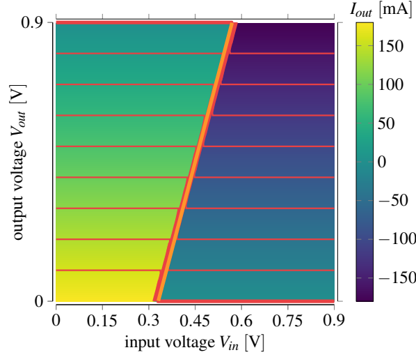
Figure 5.15: map results for opamp with a grid size of \Delta V_{in} = 1 \text{ mV} and \Delta V_{out} = 100 \text{ }\mu\text{V} . Clearly visible are the horizontal contour lines.
