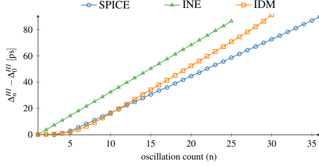
Figure 4.34: Increase of the pulse train high time compared to its initial value.
