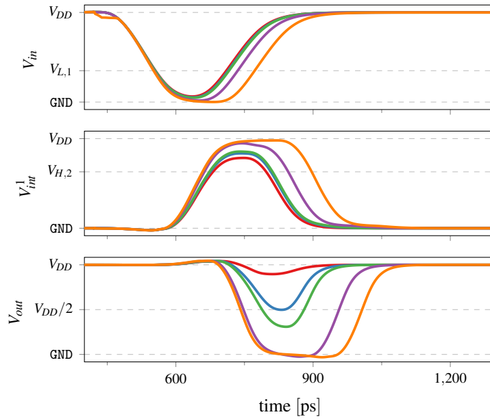
Figure 5.33: Analog simulations of the S/T cascade for input pulses. Traces initially very close show significant different output behavior due to pulse-width degradation effects, introduced by each single device.
