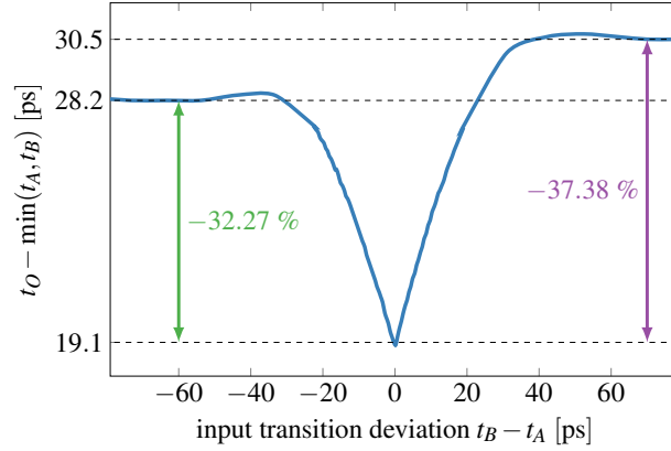
Figure 3.14: Delay to cross V_{DD}/2 at the NOR output in technology (T65) in relation to the relative input arrival times. Remarkable are the differing final values for large deviations and the local maxima for intermediate deviations (explanation in the text).
