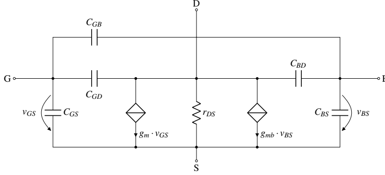
Figure 2.12: Simplified dynamic small signal circuit for an nMOS. Compared to the static circuit capacitive couplings between the terminals is added. Heavily inspired by [114] and [16].
