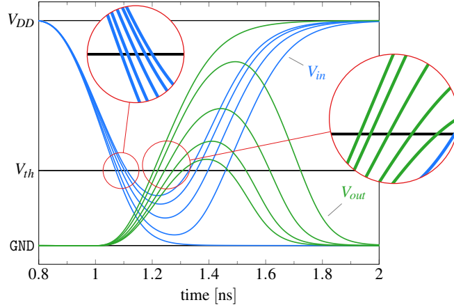
Figure 4.7: Changes of the analog in- and output waveforms for varying pulse-widths of an Inverter. For shorter input pulses, less pronounced (“shallower”) output pulses are observed leading to deviations in the relative timings ( T and \delta ).
