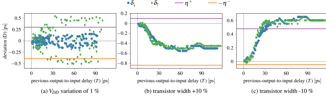
Figure 4.44: Deviation between predicted and actual V_{th} crossings for different variations. The \eta -bounds reveal good coverage for the \eta -involution model.
