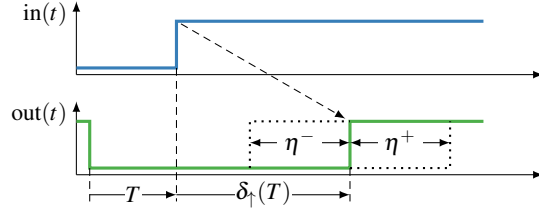
Figure 4.39: The \eta -involution channel: Non-deterministic choice of the tentative output transition after applying \delta_{\uparrow}(T) .
