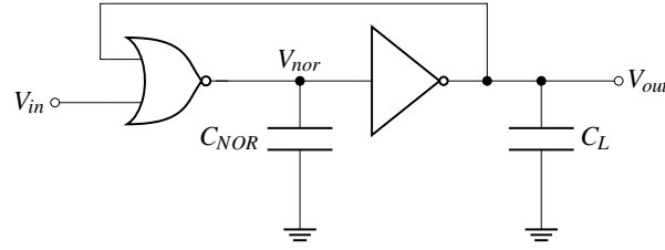
Figure 5.7: Uniform Model of an OR Loop. To reuse available models the OR-gate was split up into a NOR-gate and an Inverter.
