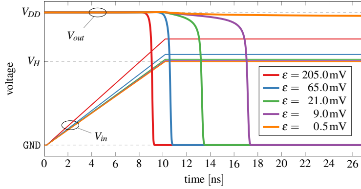
Figure 5.27: Analog HSPICE simulations of late transitions caused by a linear input traces that stop at varying values V_H + \varepsilon . The smaller \varepsilon the longer it takes until the stable output state V_{out} = \text{GND} is achieved.
