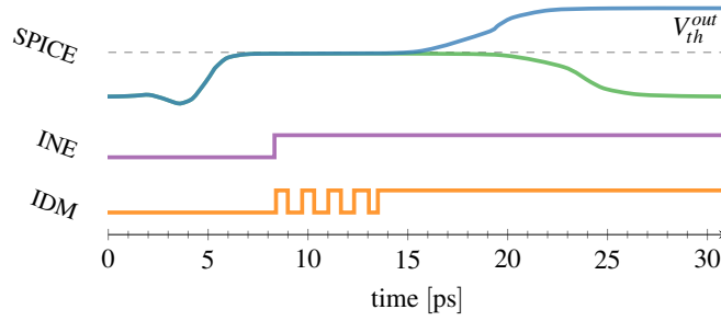
Figure 4.35: Analog and digital results of the OR Loop with direct feedback (node A).
