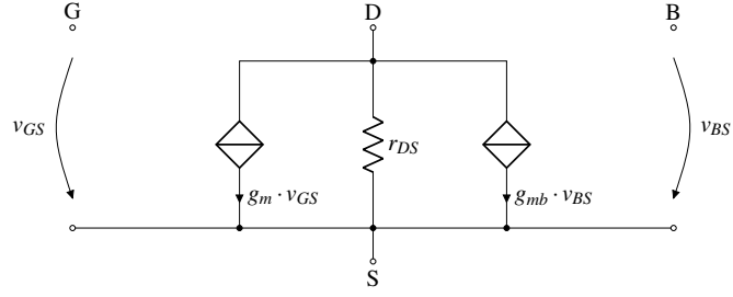
Figure 2.11: Static small signal circuit for an nMOS. The contributions of v_{GS} and v_{BS} are modeled by controlled current sources. Heavily inspired by [114] and [16].
