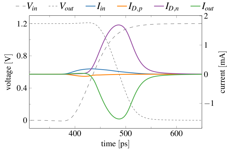
Figure 3.8: Currents inside a CMOS Inverter in technology (T65) during an in-/output transition (thin lines). The input transition induces a current I_{in} leading to I_{D,p} < 0 . This behavior stops approximately when I_{in} and I_{D,n} cross.
