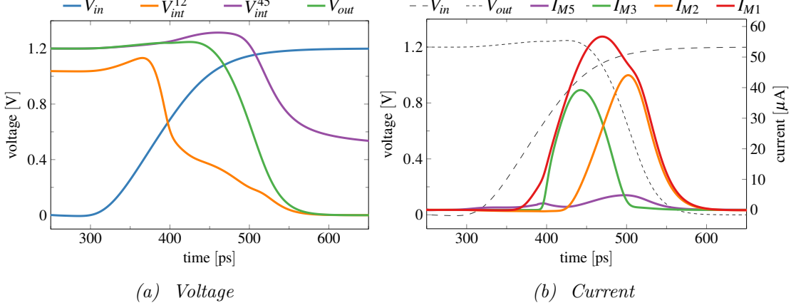
Figure 3.19: HSPICE simulation results of the S/T.
