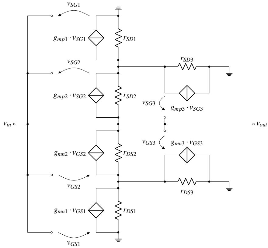
Figure 6.9: Small signal representation of the std S/T implementation. Such a model may become useful for future research such as calculating the resolution constant or optimizing an implementation.
