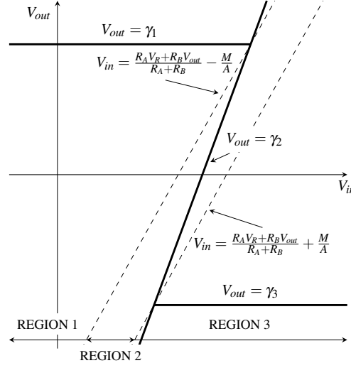
Figure 5.10: Phase plane representation ( V'_{out} in V_{in} - V_{out} plane) of the S/T as derived by Marino [146]. The bold black lines ( \gamma_1 , \gamma_2 and \gamma_3 ) denote V'_{out} = 0 .
