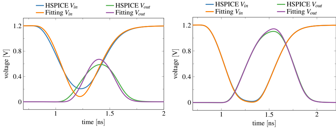
Figure 3.32: Fitting of pulses achieved by adding FRSW to HSPICE simulations. For larger pulses the fitting is much better compared to smaller ones.
