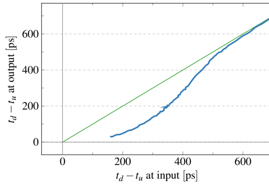
Figure 3.33: Relationship between t_d - t_u at output and input. The green line shows the first median and indicates the steep decrease of the output parameters. Most changes are caused by a shift of the second transition while the first one only slightly deviates.
