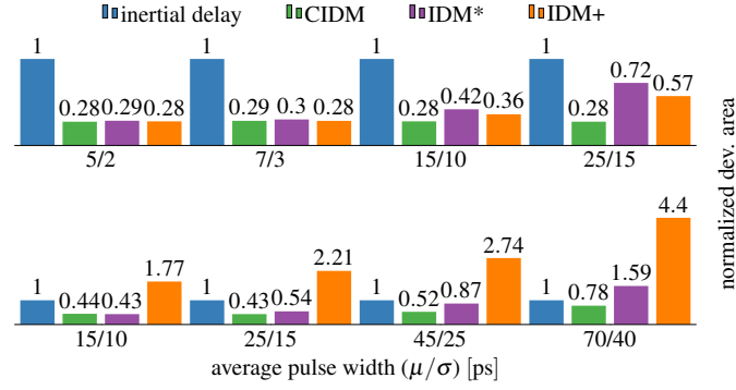
Figure 4.50: Accuracy, expressed as the normalized total deviation area of the digital predictions, relative to Spectre for the standard Inverter chain (top) and high/low threshold Inverter chain (bottom). Lower bars indicate better results.
