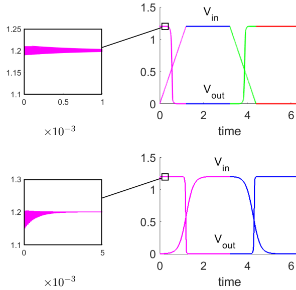
Figure 3.24: InvUni output voltage over-approximation set for V_{in} = \text{Ramp} (top) and V_{in} = \text{Sig} (bottom). Due to the fact that Uniform Model describes the behavior with a single equation the amount of states is significantly less.
