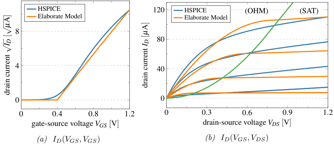
Figure 3.2: Elaborate Model approximations of the drain current I_D through an nMOS in technology (T65) (a) for V_{GS} = V_{DS} and (b) over V_{DS} for V_{GS} \in \{1.2, 1, 0.8, 0.6\} V. The current increase in (SAT) is still underestimated.
