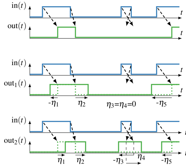
Figure 4.40: Multiple possible output behaviors for the same input trace, caused by different adversarial choices (\eta_1, \eta_2, \dots) . The output transitions that would have been caused for \eta_n = 0 are dotted. Note that different adversarial choices usually change the history and, hence, T and thus \delta(T) .
