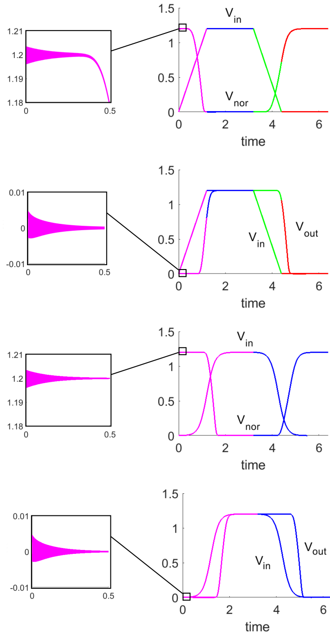
Figure 3.25: OR/NOR gate V_{nor} and V_{out} over-approximation set for V_{in} = \text{Ramp} (top half) and V_{in} = \text{Sig} (bottom half). Shown are the trajectories for V_{nor} (after the NOR gate) and V_{out} (after the Inverter).
