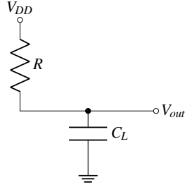
Figure 4.24: Inverter in Region 1).
