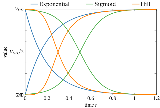
Figure 3.27: Comparison of our approximation functions. The beginning of the Exponential function is very steep and not according to reality. The other two continuously change their derivative whereat the asymmetry of the Hill function can be seen clearly. The final value is approached by all in the same fashion. Please note that the Sigmoid has a value > 0 at time zero.
