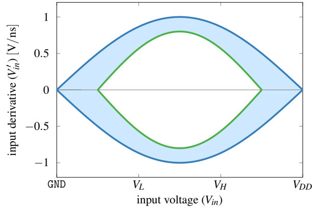
Figure 5.38: Brockett annulus specifying waveforms in the phase space, in this example for the input voltage V_{in} . For each value a region of allowed derivatives (blue area) is specified, which ensures some minimum dynamics but also limits it from above.
