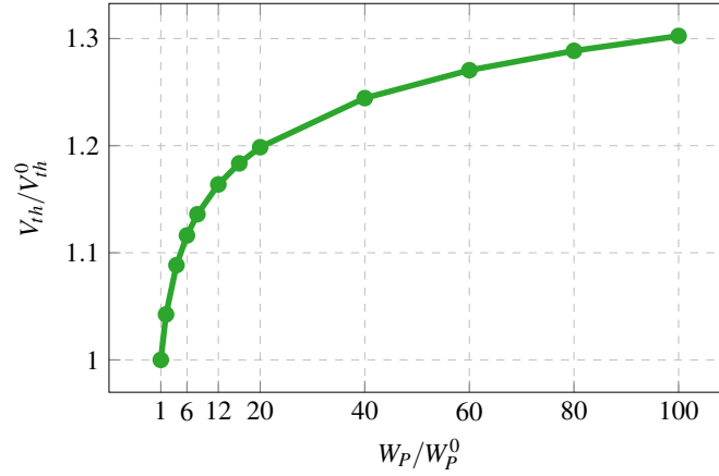
Figure 6.4: Change of the matching threshold voltage V_{th}^{in*} = V_{th}^{out*} = V_{th} by varying the width of the pMOS transistor. The change in width and threshold are related to the original values of width W_P^0 and threshold V_{th}^0 .
