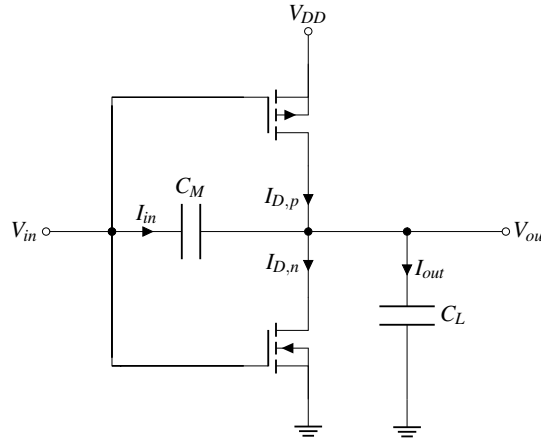
Figure 3.7: Transistor level Inverter implementation extended by coupling capacitance C_M between in- and output, which is responsible for the observed over-/undershoot effects.
