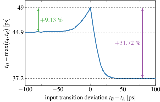
Figure 3.16: Time for the NOR output to reach V_{DD}/2 in technology (T65) after the second input reached that value, in relation to \Delta . Remarkable are the differing final values for large deviations, which depend on the initial value of V_{int}^1 (GND in these simulations).
