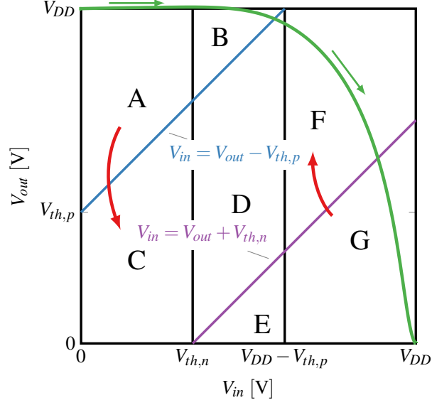
Figure 3.9: States of InvHy in the V_{in} - V_{out} plane. The green line denotes a typical rising input transition. The Basic Model was used to calculate the region boundaries. Red arrows indicate physically unreasonable transitions.
