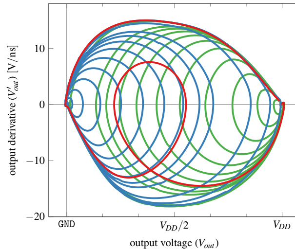
Figure 6.7: Phase space representation of pulses applied to a Buffer using technology (T65). Shown are up-pulse (blue), down-pulses (green) and a single trace consisting of four transitions (red), which was used to evaluate the approach. By picking reasonable switching points the latter can be approximated closely.
