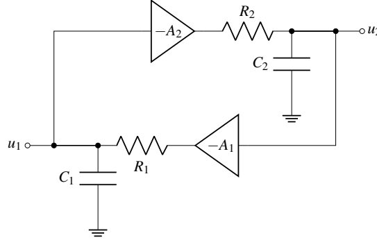
Figure 5.13: Simplified feedback loop model with active feedback path.
