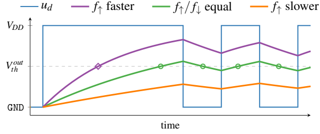
Figure 4.33: Analog waveform u_r of the IDM for various combinations of f_{\uparrow} and f_{\downarrow} .
