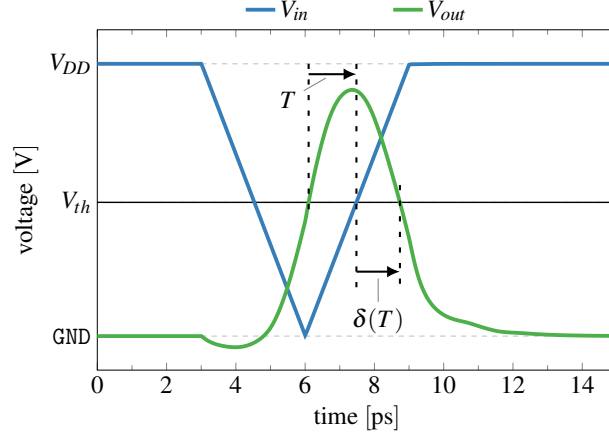
Figure 4.3: Characterization procedure of the DDM, showing the input slopes ( V_{in} ) and output trajectory ( V_{out} ) of an Inverter gathered from HSPICE simulations using technology (T15). T and \delta are extracted as shown to determine \delta(T) numerically.
