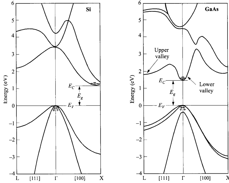
Figure 2.3: Band diagram for Silicon (left) and GaAs (right) showing the CB (top) and VB (bottom). [100] and [111] correspond to two different directions of the wave vector k . Taken from [73, p. 14]
