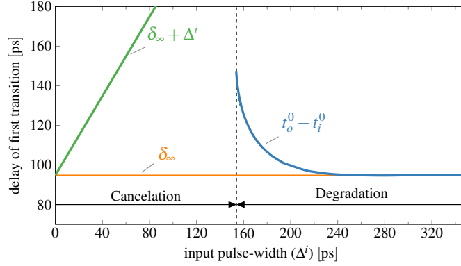
Figure 4.10: Variations in the delay of the first transition. The bound \delta_\infty + \Delta^i must not be exceeded, as this would result, in the case of an input glitch, in a value T < -\delta_\infty .
