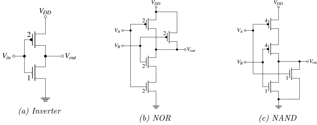
Figure 6.5: Transistor sizing of various gates to have the same conductivity as the Inverter. Taken from [109].
